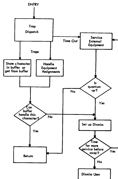
Figure 1 General Flow Diagram of Executive Routine
